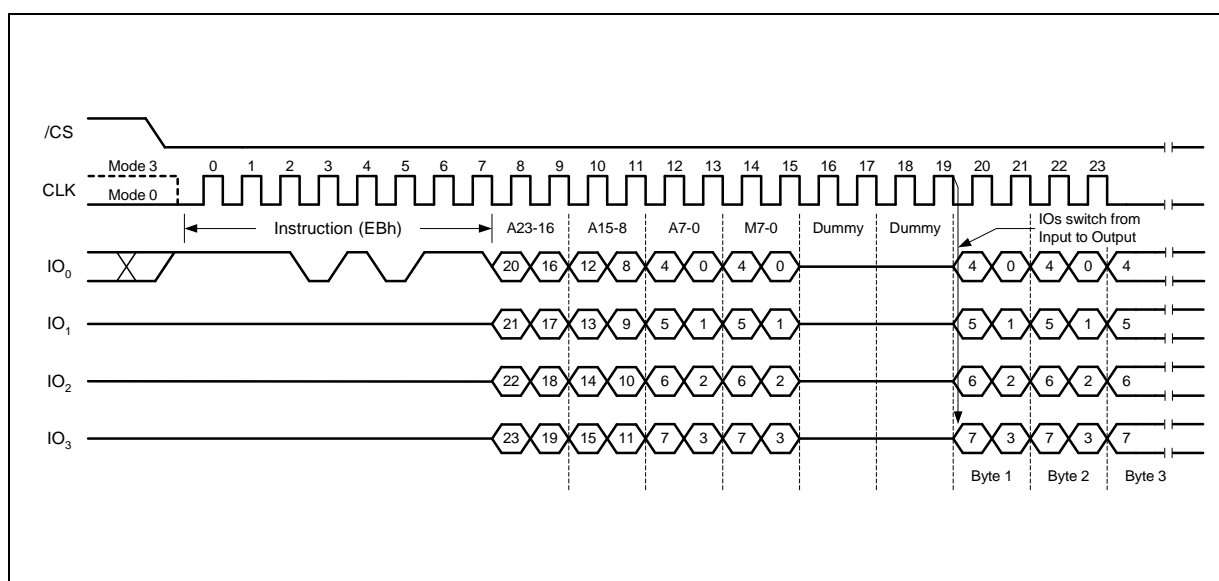
Figure 24a. Fast Read Quad I/O Instruction (M5-4=Fxh, SPI Mode)
