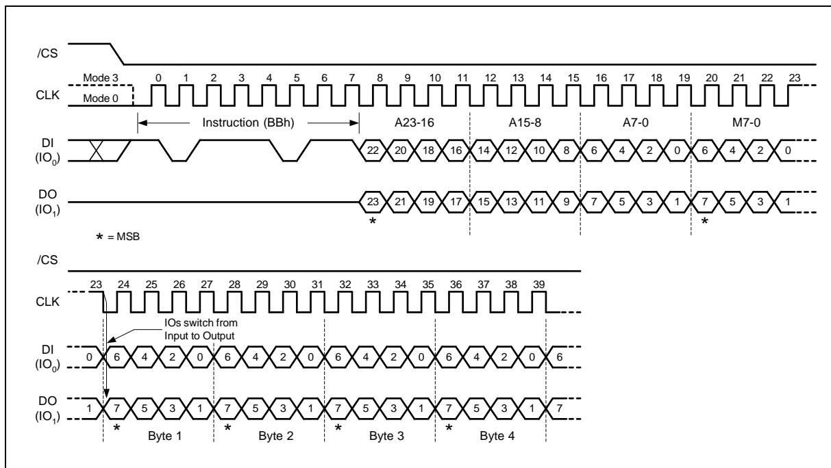
Figure 22a. Fast Read Dual I/O Instruction (M5-4=Fxh., SPI Mode only)
