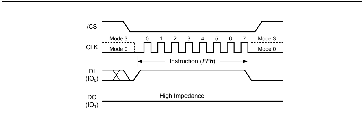
Figure 5a. Device Reset Instruction
