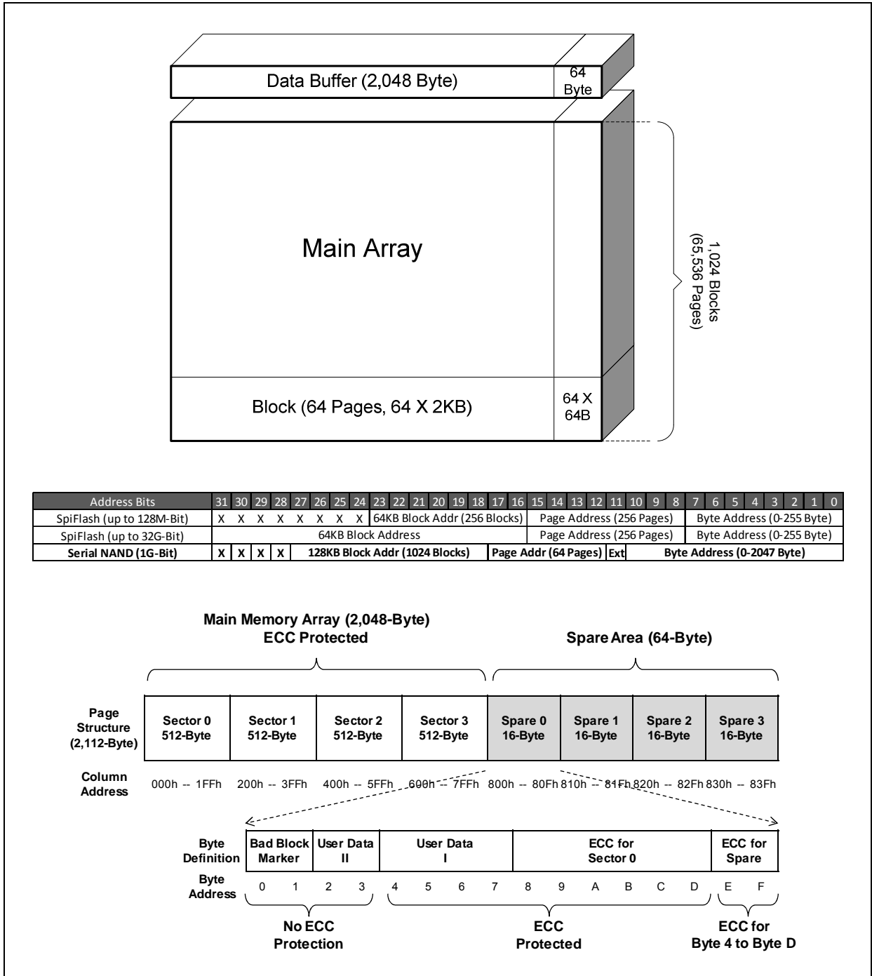
Figure 2. W25N01GV SpiNAND Flash Memory Architecture and Addressing
