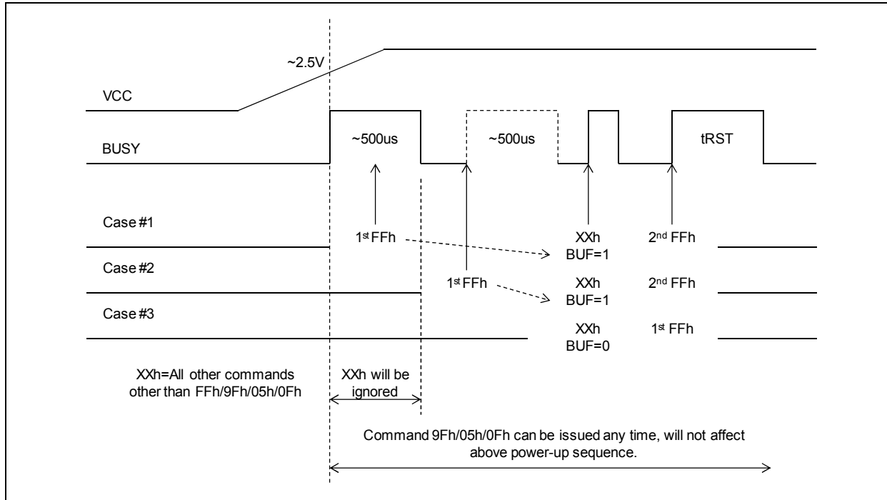
Figure 5b. Device Reset Instruction Timing Sequence
