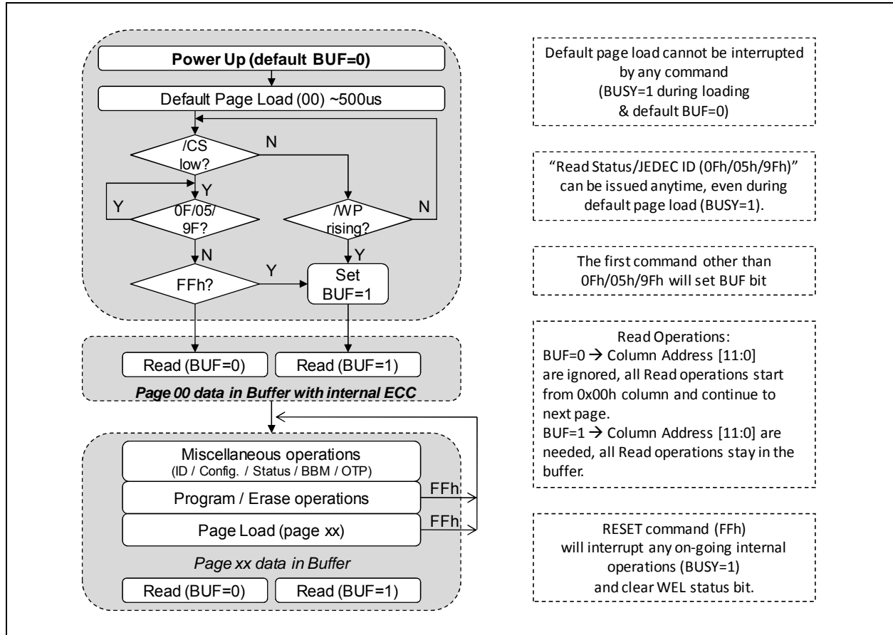
Figure 3. W25N01GV SpiNAND Flash Memory Operation Diagram
