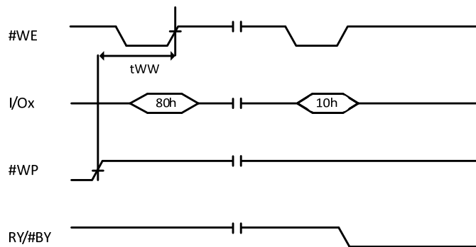
Figure 9-14 Program Enable
