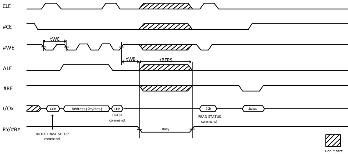
Figure 11-15 Block Erase
