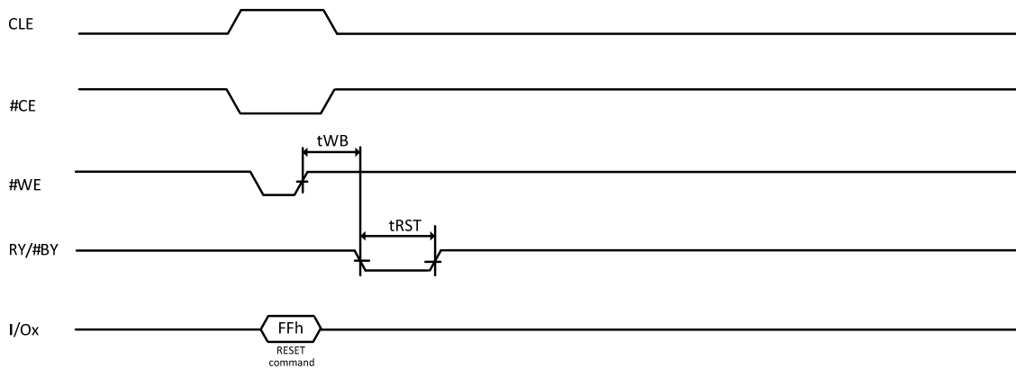
Figure 9-11 Reset Operation
