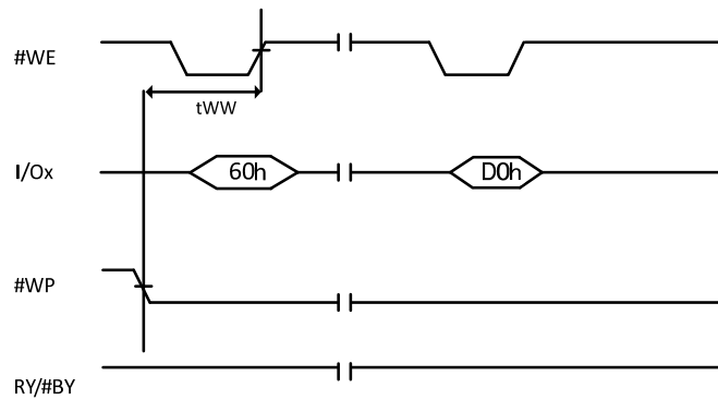
Figure 9-13 Erase Disable
