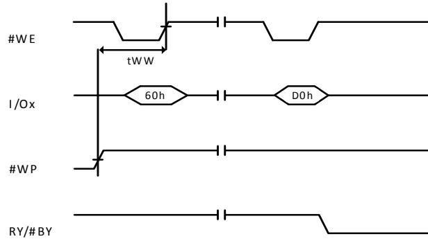
Figure 9-12 Erase Enable
