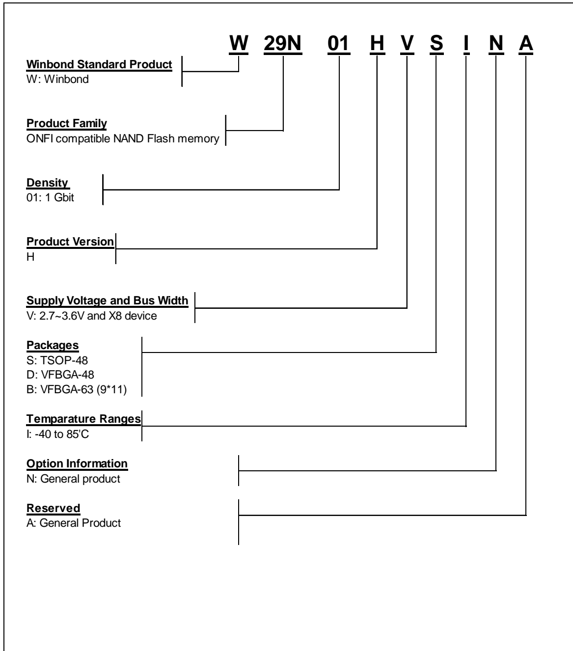
Figure 14-1 Ordering Part Number Description
