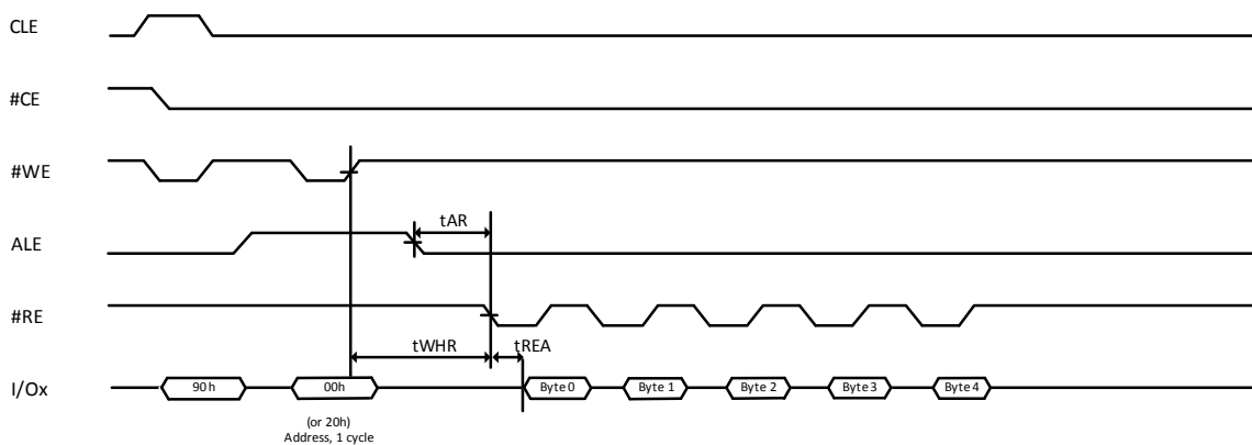
Figure 9-3 Read ID
