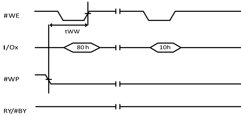
Figure 9-15 Program Disable
