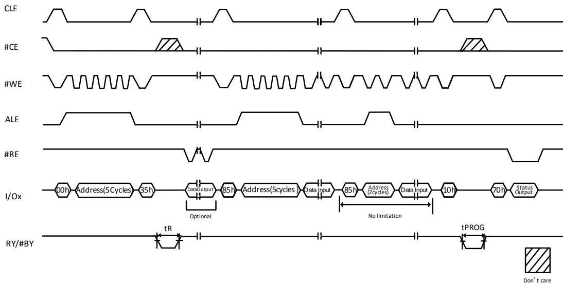
Figure 9-9 Copy Back Operation with Random Data Input
